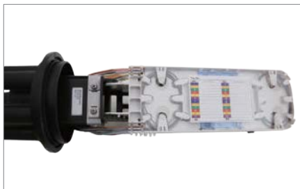
In-line connection
